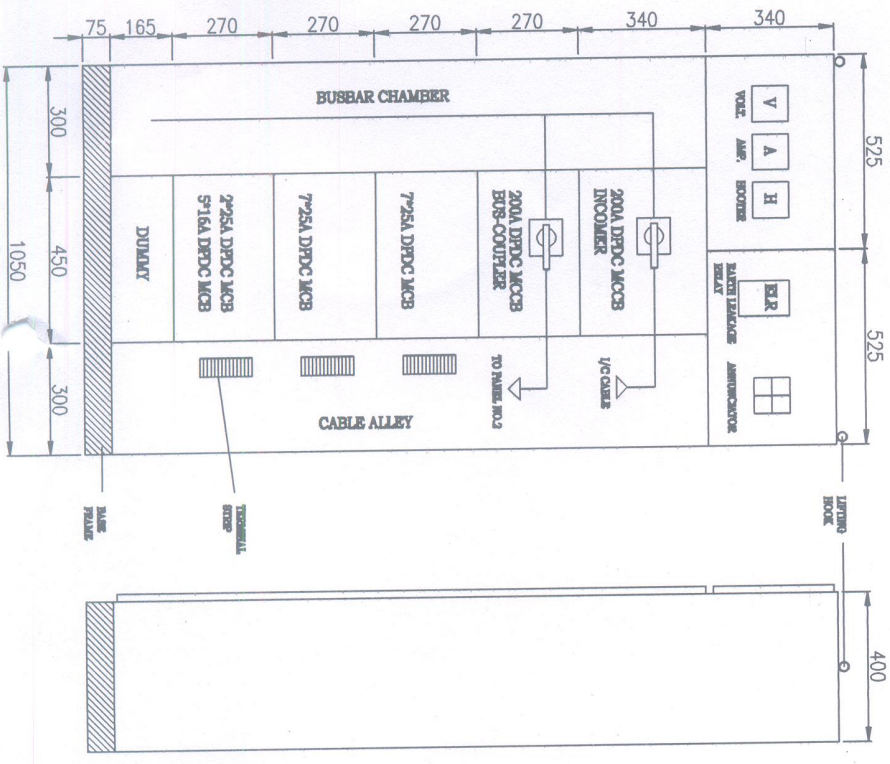
200V-300AH DCDB
